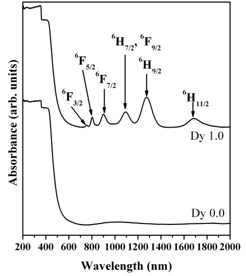
Fig. 4. Typical absorption spectra of bismuth-borate glass with 1.0 mole% Dy_2O_3 doping and without Dy_2O_3 doping.
