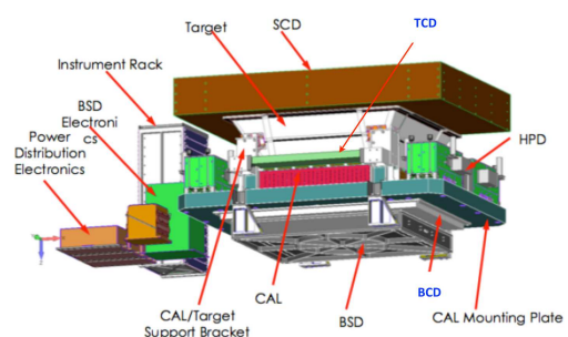
Fig. 1: ISS-CREAM instrument.
