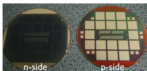
Fig. 5: Photograph of the photo-diodes on 6-inch and 650 \mu\text{m} thickness silicon wafer.
