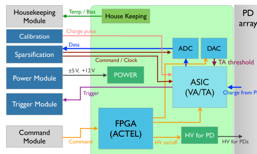
Fig. 8: Signal flows in the T/BCD readout electronics and ISS-CREAM common electronics.
