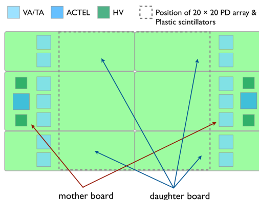
Fig. 7: Design of T/BCD electronics. There are two mother boards and four daughter boards for each of the TCD and BCD.
