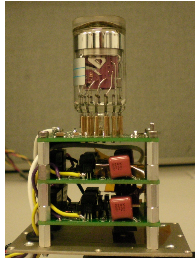
Fig. 2: A PMT assembly. The R1924A plugs in to a socketed high voltage divider board (top board). The two bottom boards switch the potential applied to dynodes 1 and 2 from -12 V during the initial calorimeter shower to their full high voltage values within 300 ns.
